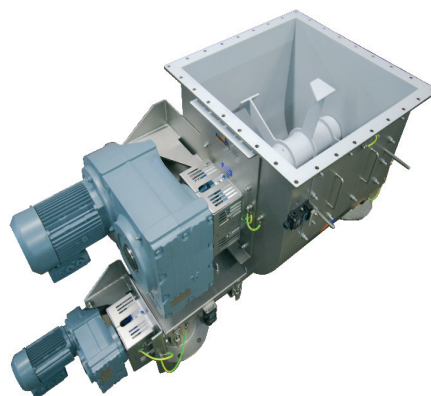
Buffering, homogenizing and measuring out clinging products
