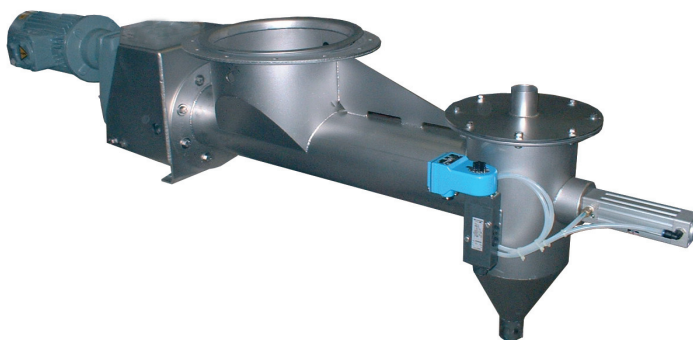
Small dosing screw with overhead valve for measuring out granulate directly into pneumatic transport.
