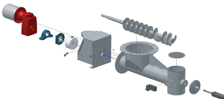
Heavy-duty version of dosing screw with overhead valve, with double speed for accurate dosing.
