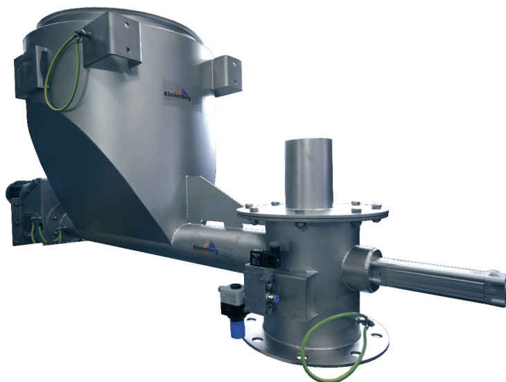
Pneumatic dosing screw with overhead valve with 1000-litre hopper; zone 20 internally, zone 22 externally.
