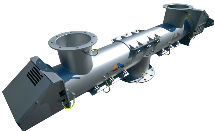
Tube conveyor with inspection hatches
