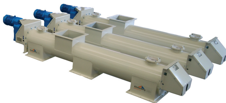
Tube conveyor fitted with overflow prevention, one inlet and 3 outlets.
