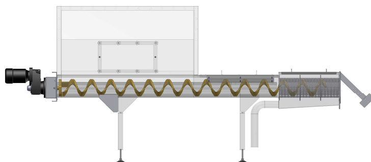
Dewatering screw press for paper sludge
