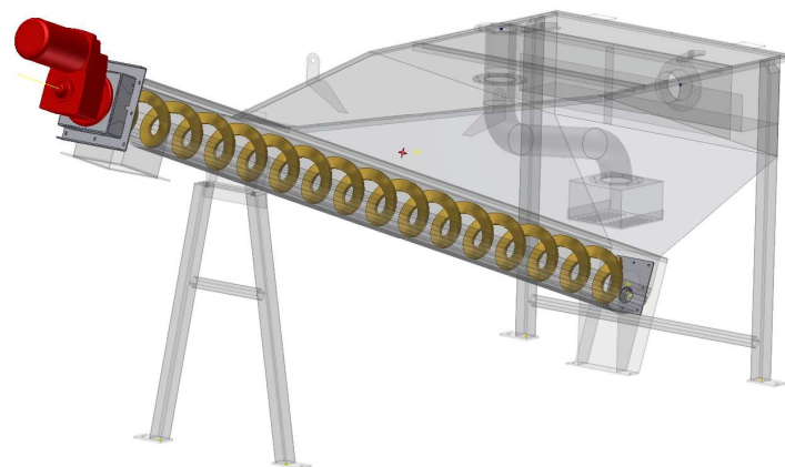
3D layout of a sand separator
