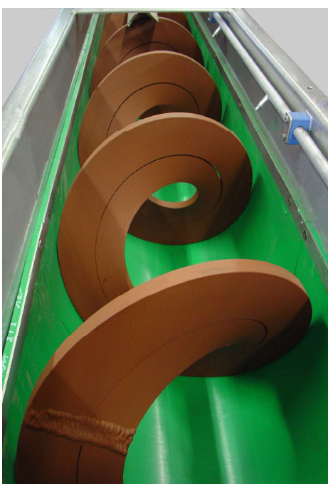
Shaftless screw conveyor with housing made of stainless steel 304, equipped with an HDPE-1000 liner and spray nozzles
